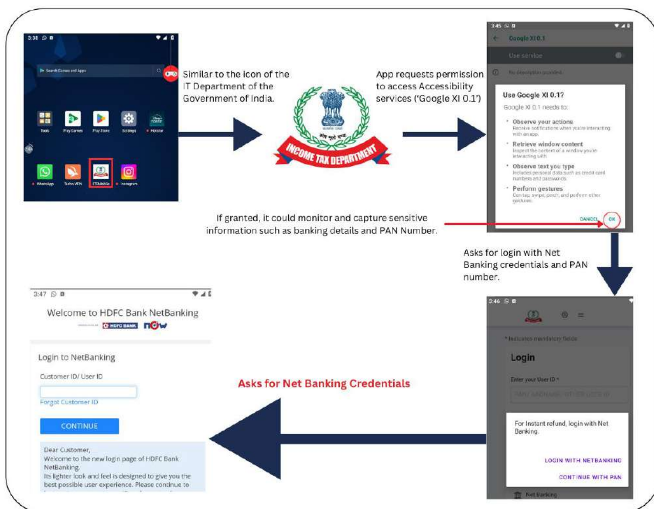
Fig. 2.1 A case of a malicious app
